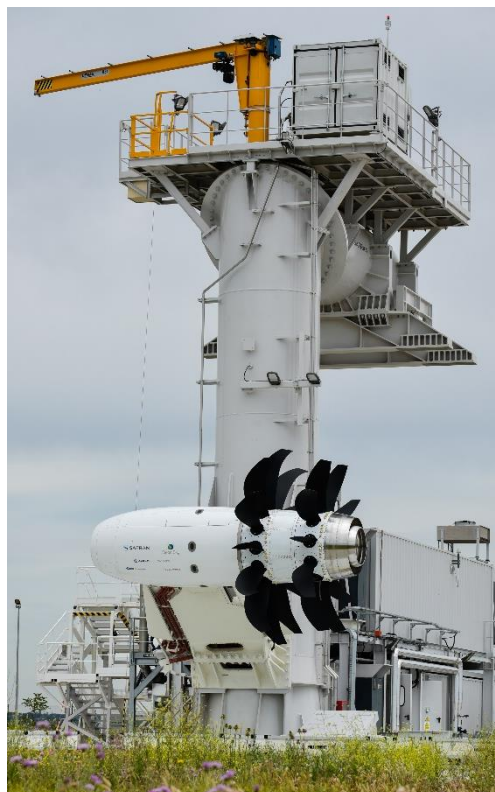
Open Rotor engine
